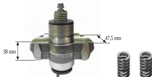
Caliper Adj. Mech. Housing (Thick) 80,4mm (with Pin) Kaliper Ayar Mek. Yatađý (Kalýn) 80,4mm/114mm (Pimli)
